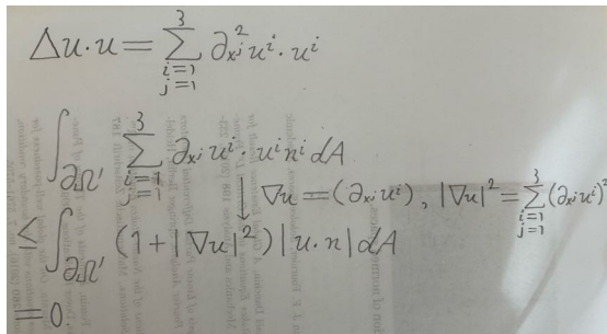
Energy inequality.
